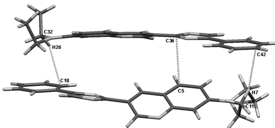
Fig. 3. Intermolecular C—H⋯π and π⋯π interactions in 1a and 1b .
