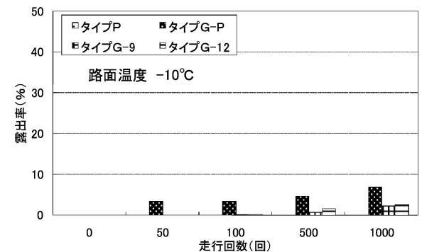
図4.4 路面露出率 (氷板・ -10^{\circ}\text{C} )
