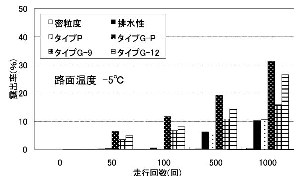
図4.3 路面露出率 (氷板・ -5^{\circ}\text{C} )
